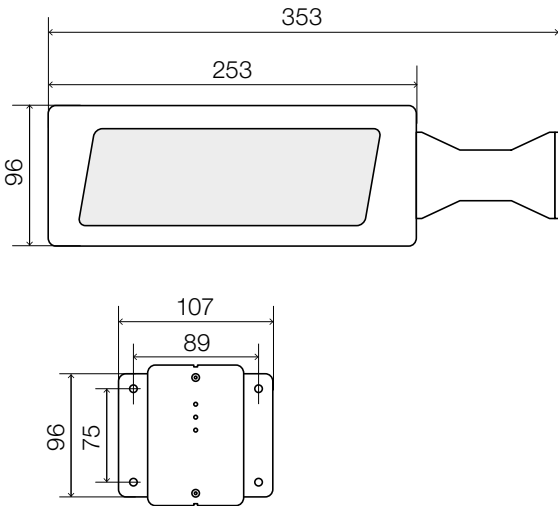
1 Wall mounting LUMEX 5
