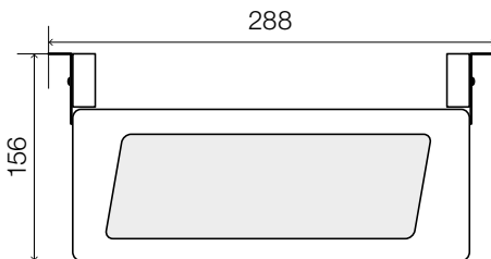
2 Ceiling mounting LUMEX 5
