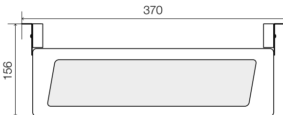
Ceiling mounting LUMEX 5-S
